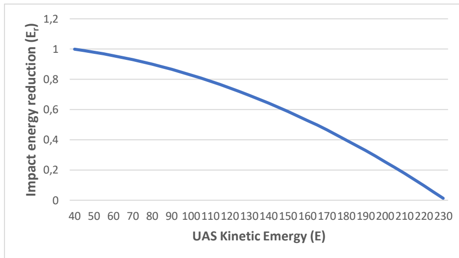
Figure 5: Quadratic relationship between the E_r and E at impact
